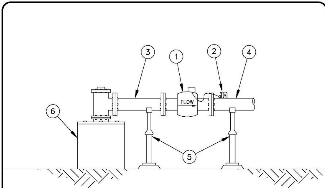
Figure 4. Detail of a Typical Flowmeter Installation
